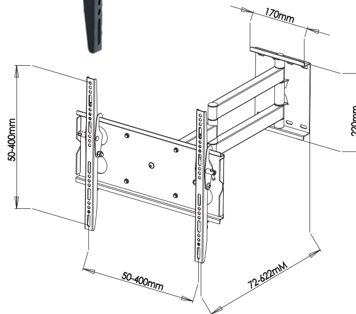
(Schematic Diagram)
